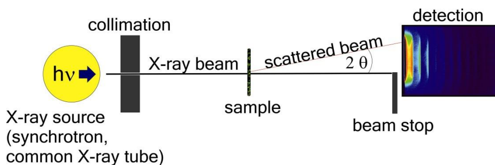
Figure 4: Measurement principle of SAXS
