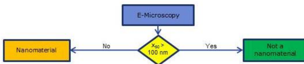
Figure 14: Tier 2 classification
