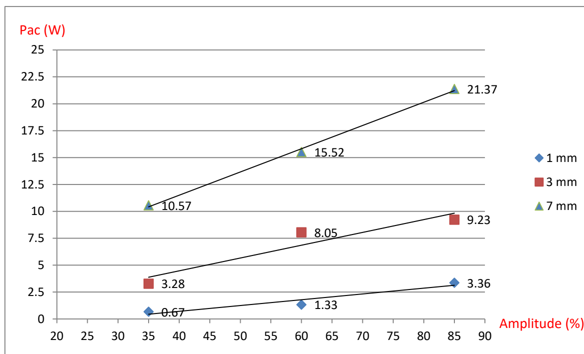
Figure 3: Example of calorimetrically determined sonication power
