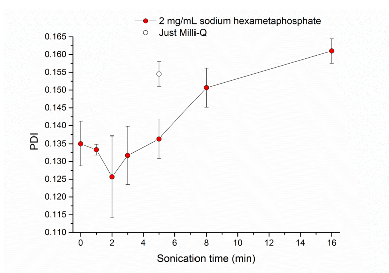
Figure 4: PDI values obtained by DLS for IRMM-387 – BaSO_4 (ultrafine grade) suspensions in MilliQ water (N=2) and 2\text{mgmL}^{-1} hexametaphosphate (N=3) prepared at different probe sonication times
