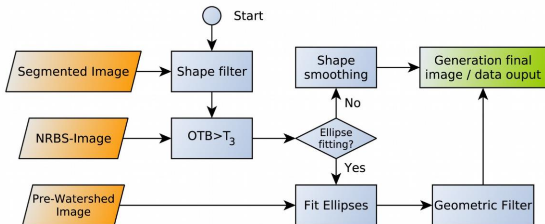
Figure 6: Post-processing pipeline
