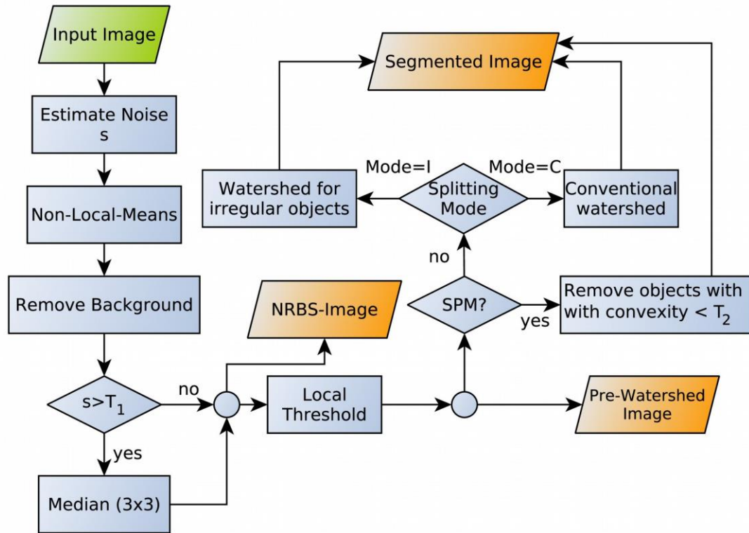
Figure 5 Pre-processing pipeline
