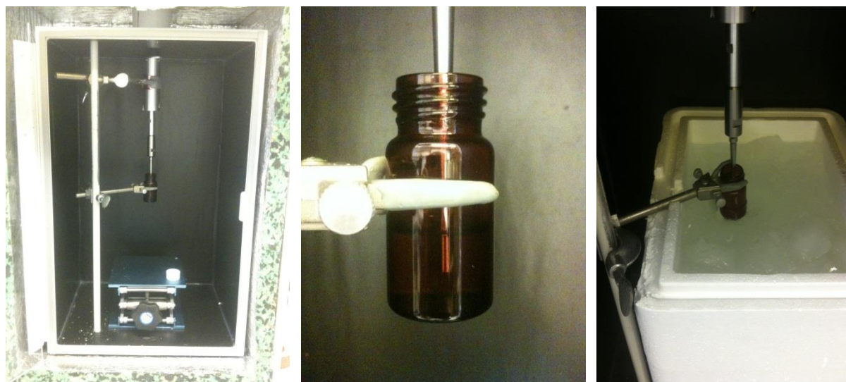
Figure 2: Ultrasonic probe sonication setup for dispersion of NM powders
