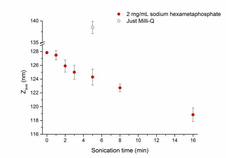
Figure 3: Z_{ave} values obtained by DLS for IRMM-387 – BaSO_4 (ultrafine grade) suspensions in MilliQ water (N=2) and 2\text{mgmL}^{-1} hexametaphosphate (N=3) prepared at different probe sonication times
