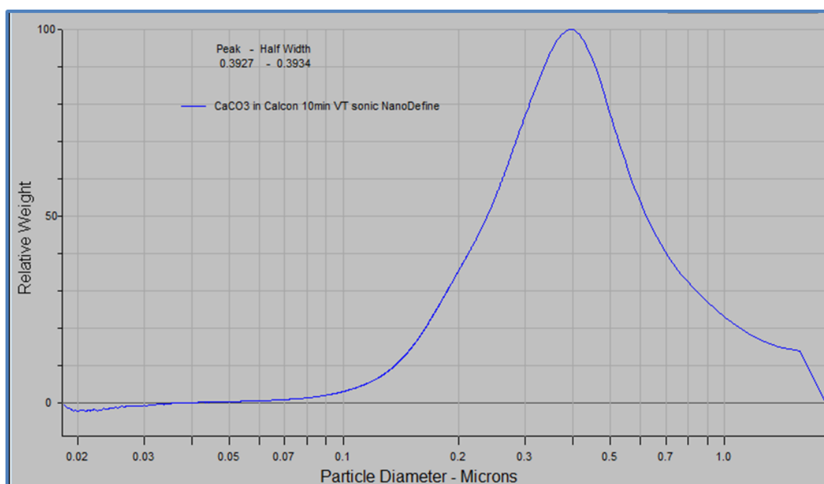
Figure 4: Typical particle size distribution of dispersed \text{CaCO}_3 determined by CLS
